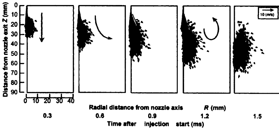
Fig. 9 Temporal change of spatial distribution of droplets velocity ( p_{inj} = 600 bar, t_{inj} = 1.2 ms)
