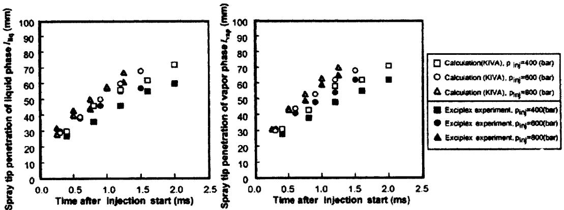
Fig. 8 Comparison of spray tip penetration by means of simulation analysis with experiment results
