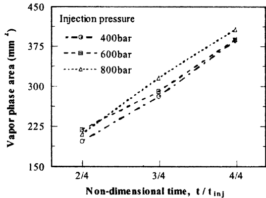
Fig. 6 Temporal change of vapor phase area
