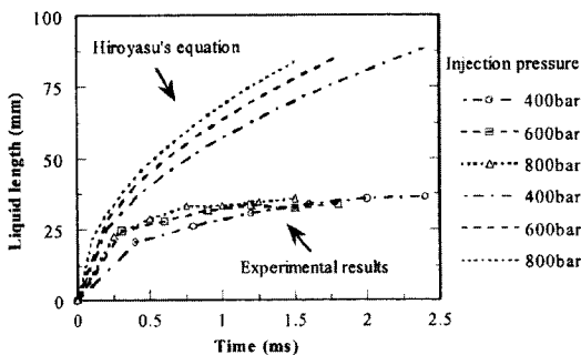
Fig. 5 Liquid length (ms) compared with Hiroyasu's equation
