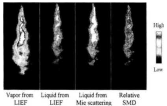
Fig. 2 Spray images and relative SMD distribution
